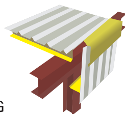
GABLE FLASHING
